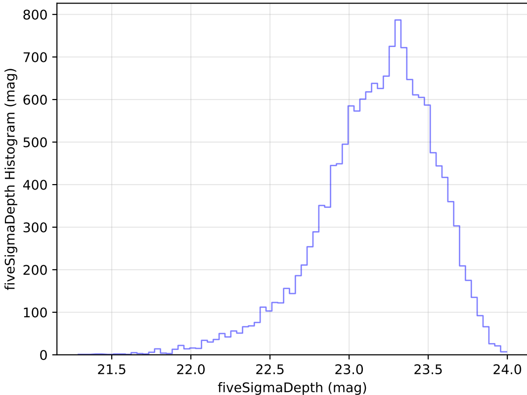
internal_u_expt27_nscale0.9v3.4_10yrs Yr 1 u band: fiveSigmaDepth Histogram
