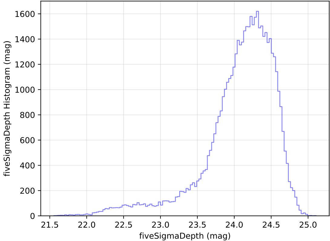
internal_u_expt27_nscale0.9v3.4_10yrs Yr 1 r band: fiveSigmaDepth Histogram
