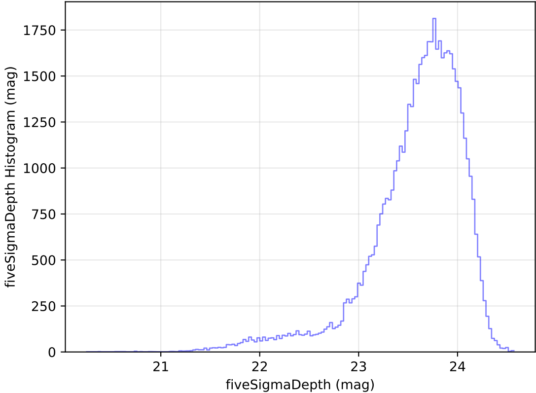
internal_u_expt27_nscale0.9v3.4_10yrs Yr 1 i band: fiveSigmaDepth Histogram
