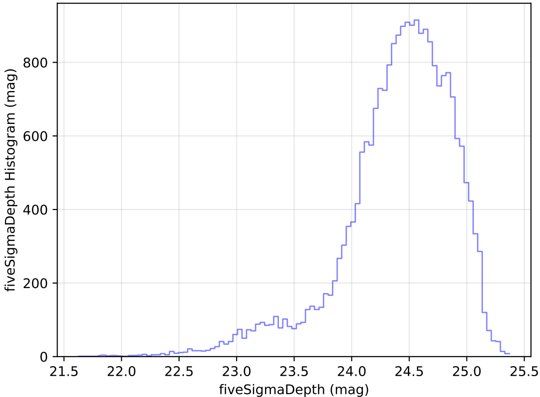
internal_u_expt27_nscale0.9v3.4_10yrs Yr 1 g band: fiveSigmaDepth Histogram
