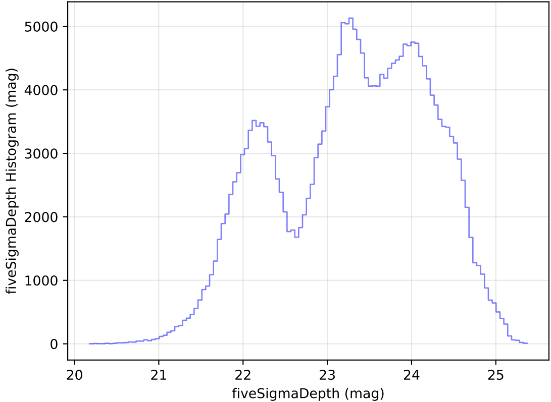
internal_u_expt27_nscale0.9v3.4_10yrs Yr 1 all bands: fiveSigmaDepth Histogram
