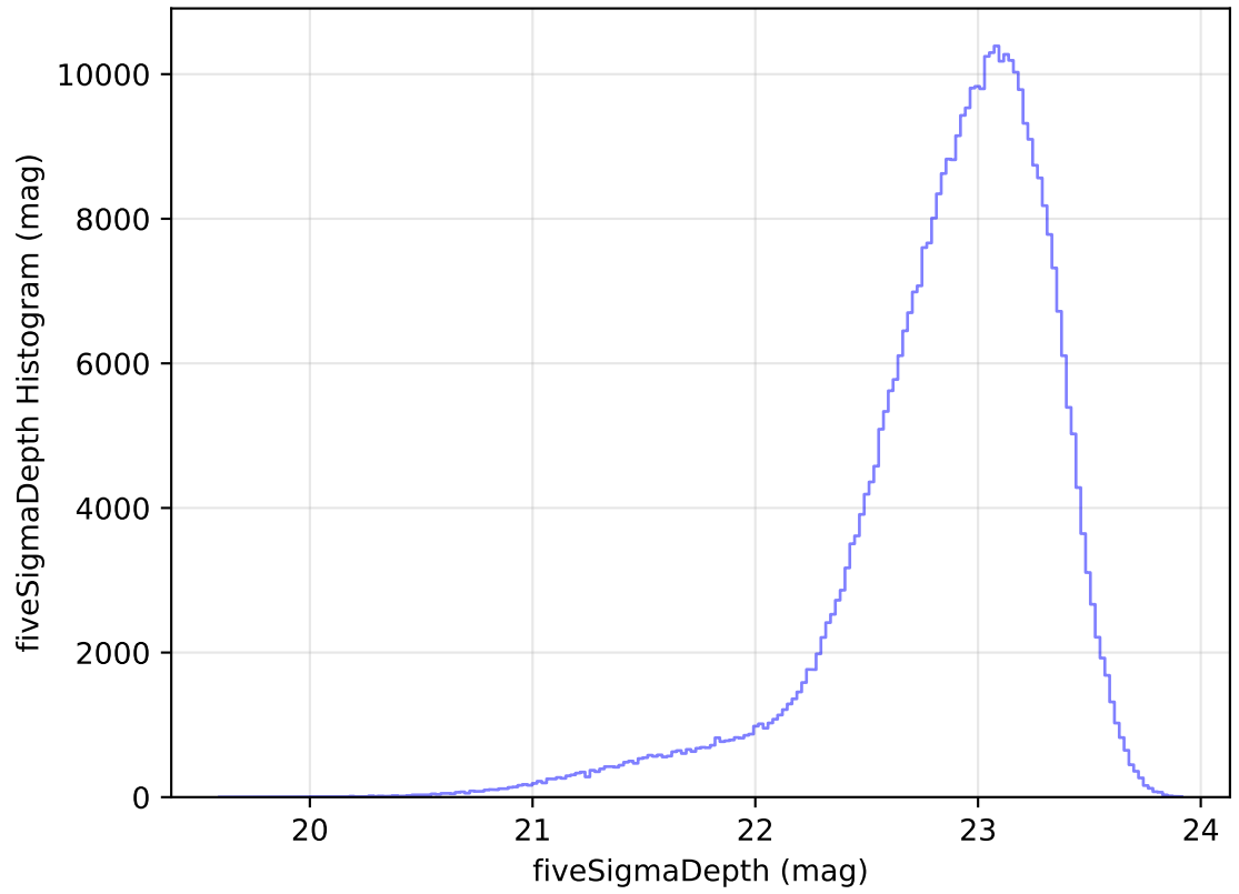
internal_u_expt27_nscale0.9v3.4_10yrs WFD z band: fiveSigmaDepth Histogram
