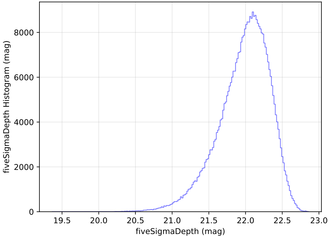
internal_u_expt27_nscale0.9v3.4_10yrs WFD y band: fiveSigmaDepth Histogram
