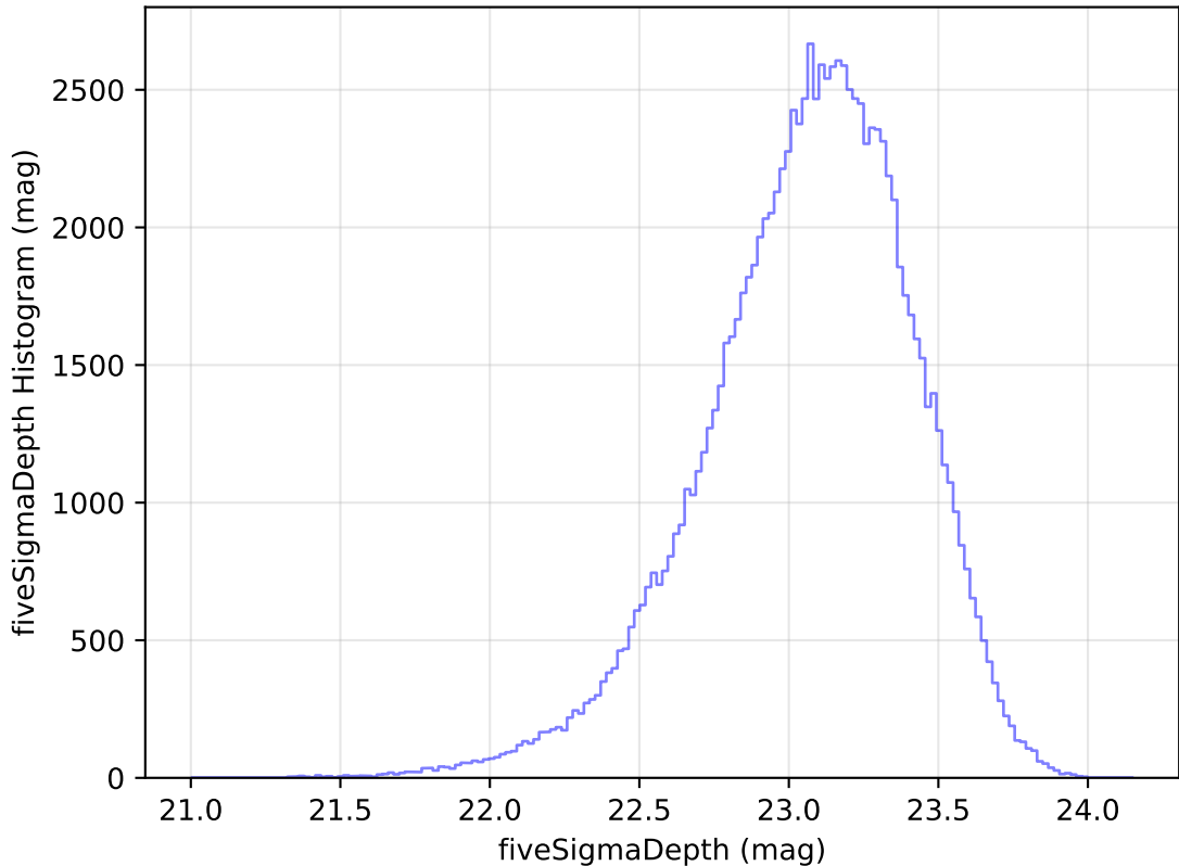
internal_u_expt27_nscale0.9v3.4_10yrs WFD u band: fiveSigmaDepth Histogram
