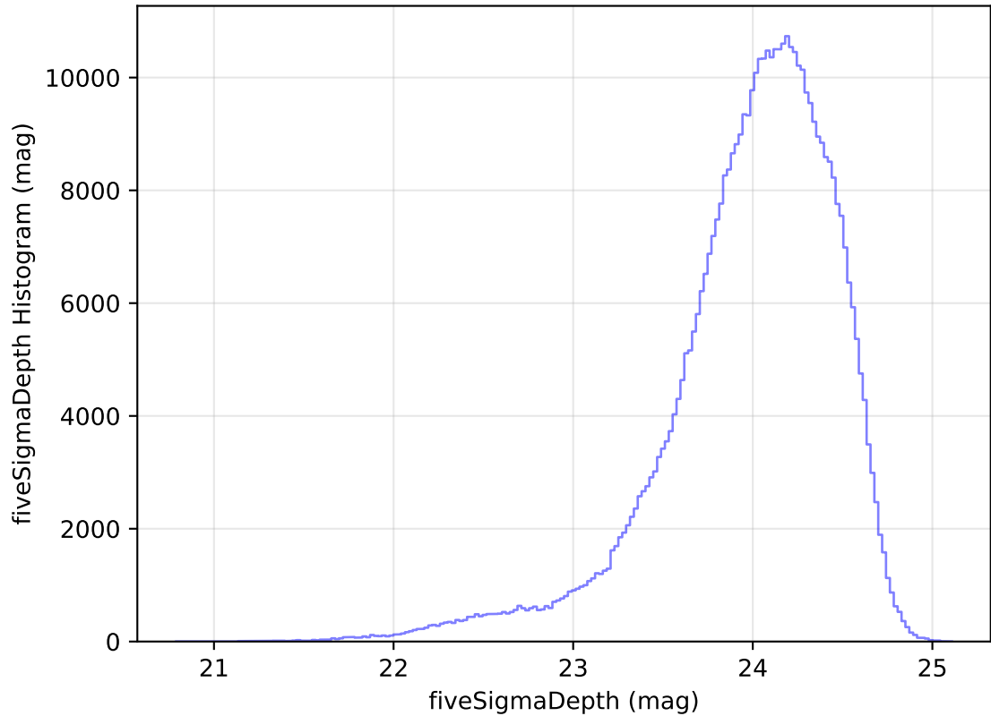
internal_u_expt27_nscale0.9v3.4_10yrs WFD r band: fiveSigmaDepth Histogram
