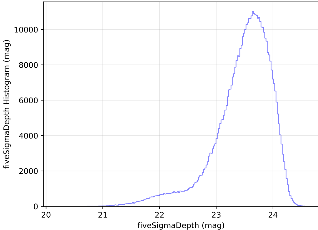
internal_u_expt27_nscale0.9v3.4_10yrs WFD i band: fiveSigmaDepth Histogram
