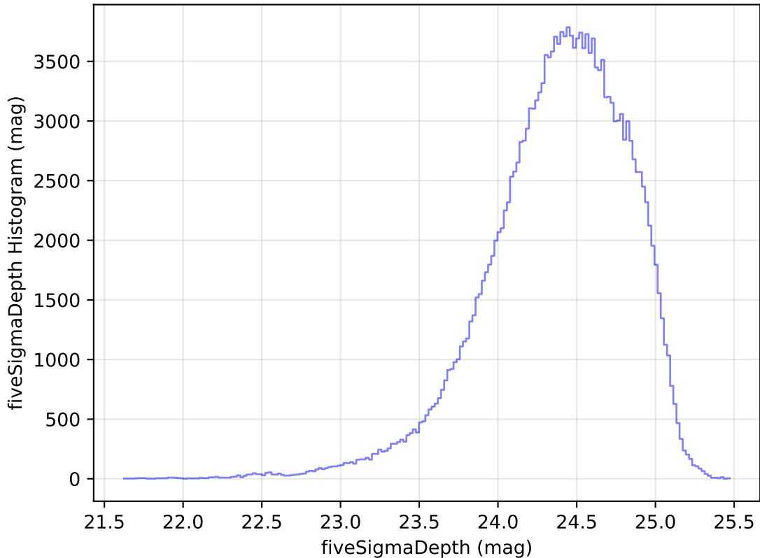
internal_u_expt27_nscale0.9v3.4_10yrs WFD g band: fiveSigmaDepth Histogram
