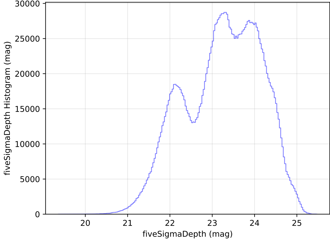
internal_u_expt27_nscale0.9v3.4_10yrs WFD all bands: fiveSigmaDepth Histogram
