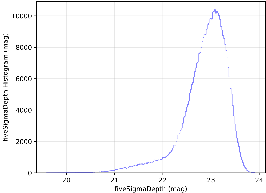
internal_u_expt27_nscale0.9v3.4_10yrs All sky z band: fiveSigmaDepth Histogram
