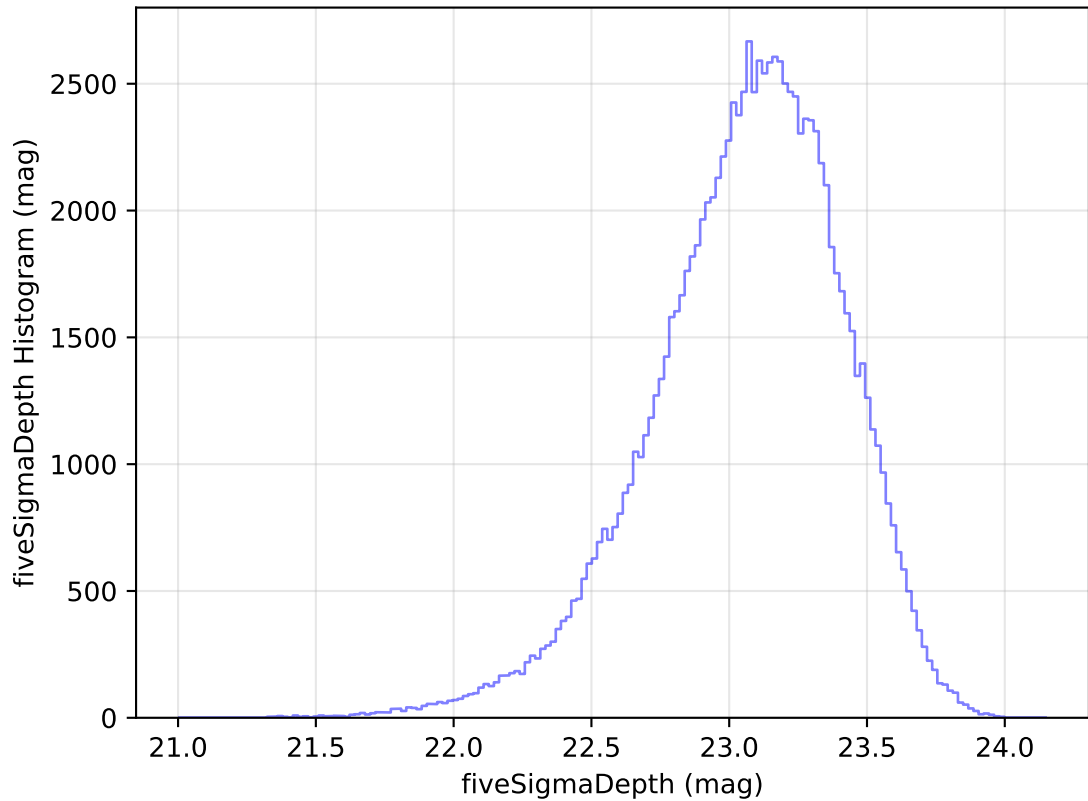
internal_u_expt27_nscale0.9v3.4_10yrs All sky u band: fiveSigmaDepth Histogram
