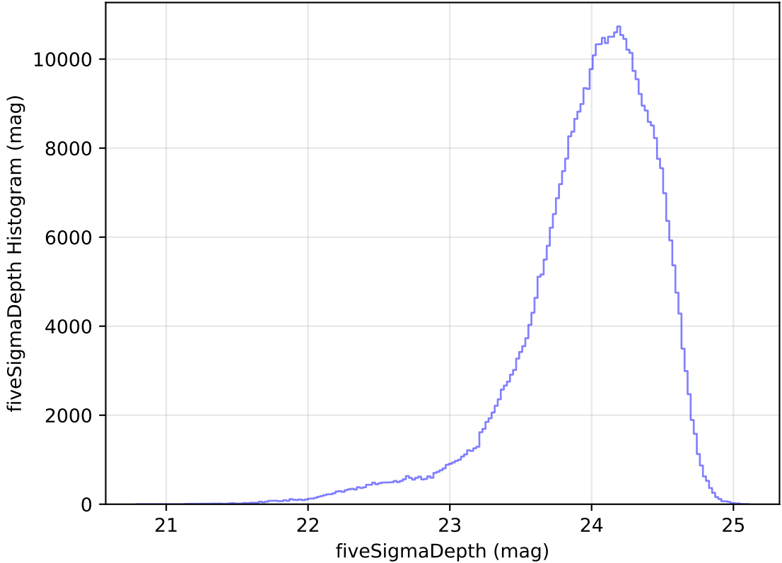
internal_u_expt27_nscale0.9v3.4_10yrs All sky r band: fiveSigmaDepth Histogram
