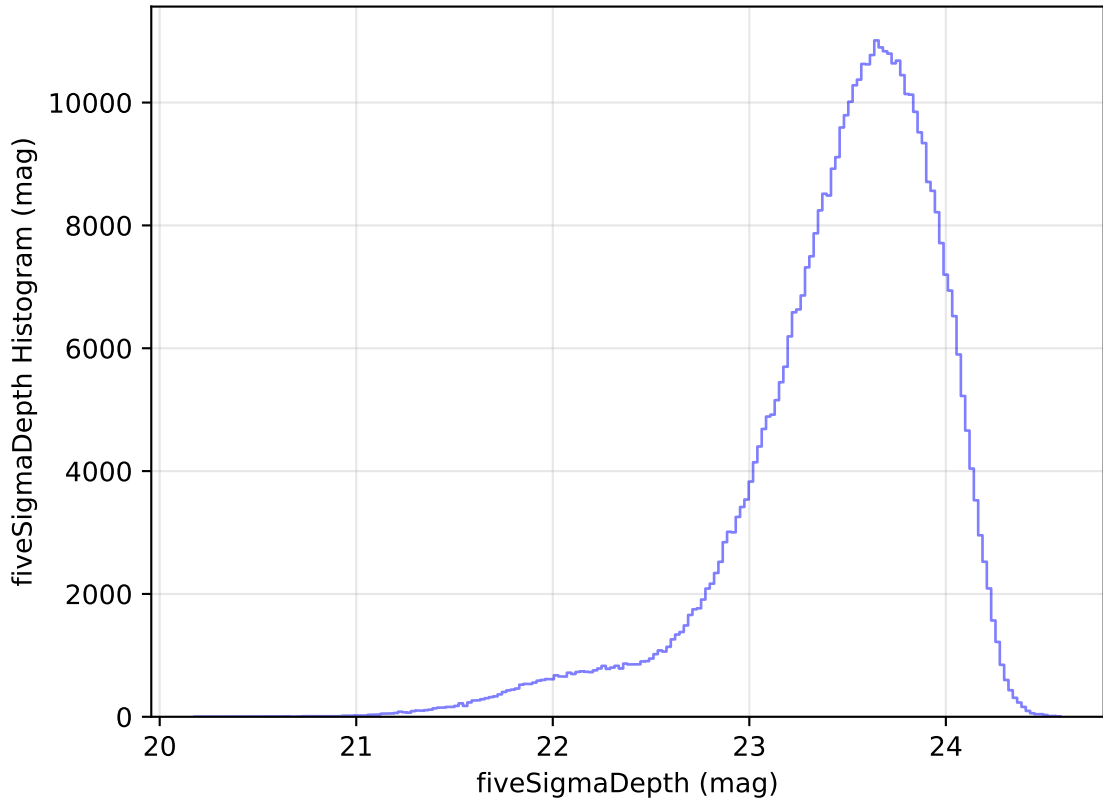
internal_u_expt27_nscale0.9v3.4_10yrs All sky i band: fiveSigmaDepth Histogram
