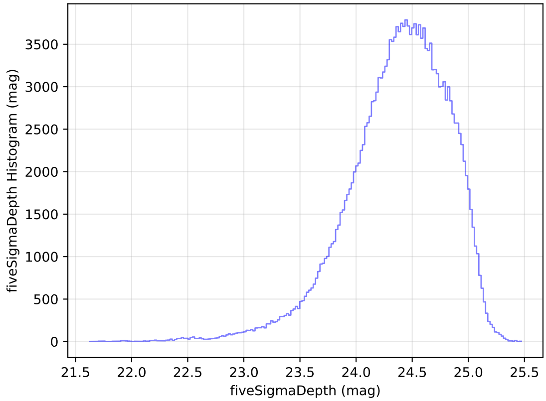
internal_u_expt27_nscale0.9v3.4_10yrs All sky g band: fiveSigmaDepth Histogram
