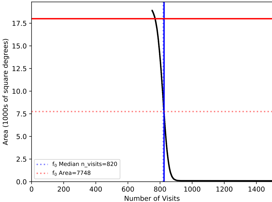
internal_u_expt27_nscale0.9v3.4_10yrs WFD: fO
