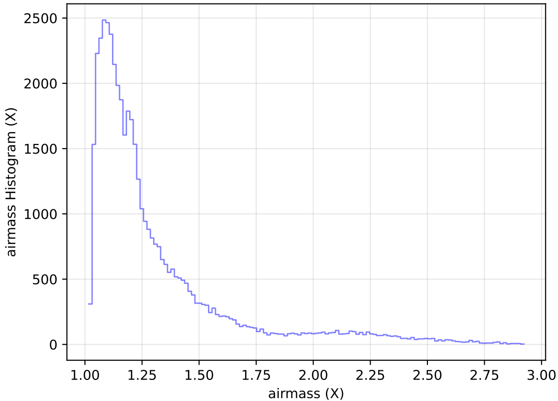
internal_u_expt27_nscale0.9v3.4_10yrs Yr 1 z band: airmass Histogram
