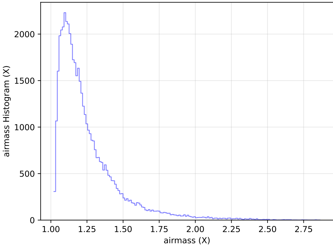
internal_u_expt27_nscale0.9v3.4_10yrs Yr 1 y band: airmass Histogram
