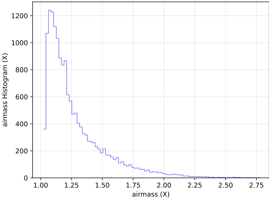
internal_u_expt27_nscale0.9v3.4_10yrs Yr 1 u band: airmass Histogram
