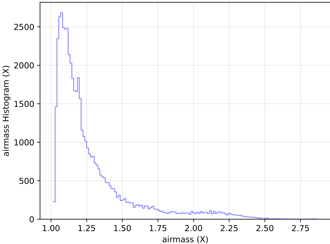
internal_u_expt27_nscale0.9v3.4_10yrs Yr 1 r band: airmass Histogram
