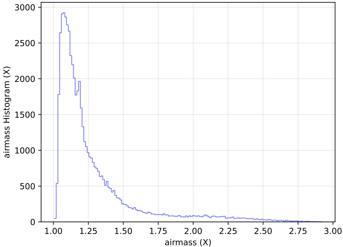
internal_u_expt27_nscale0.9v3.4_10yrs Yr 1 i band: airmass Histogram
