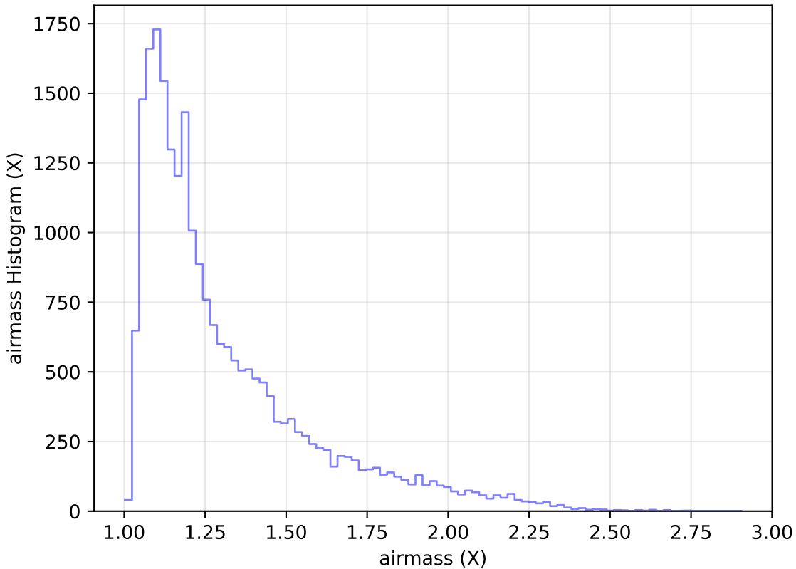
internal_u_expt27_nscale0.9v3.4_10yrs Yr 1 g band: airmass Histogram
