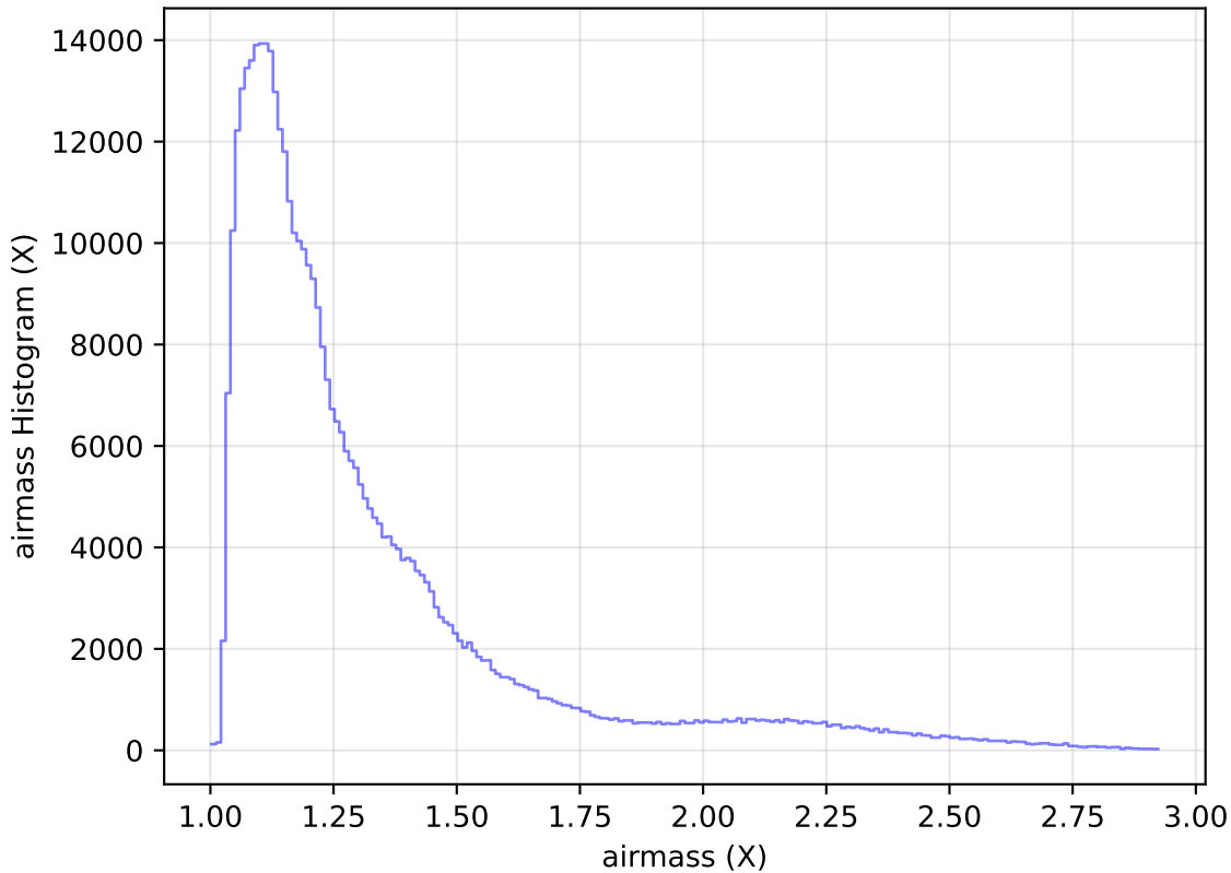
internal_u_expt27_nscale0.9v3.4_10yrs WFD z band: airmass Histogram
