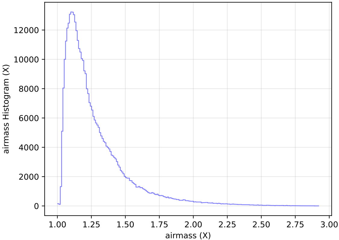
internal_u_expt27_nscale0.9v3.4_10yrs WFD y band: airmass Histogram
