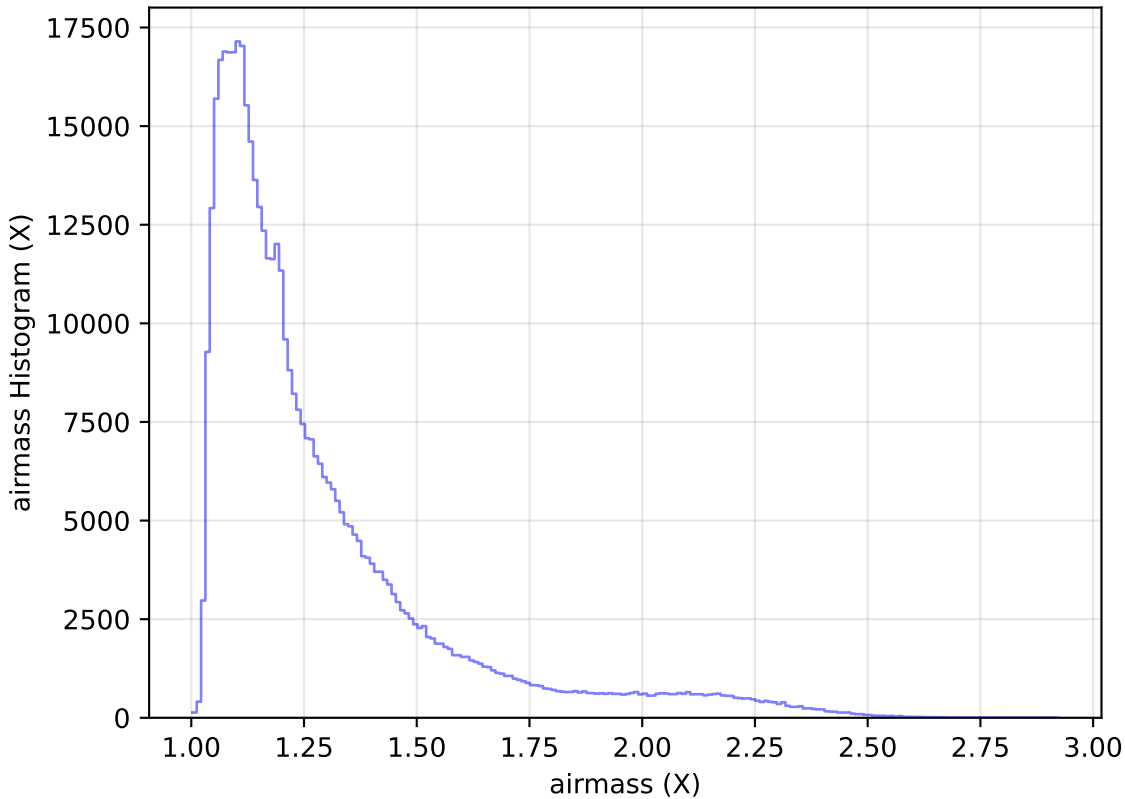
internal_u_expt27_nscale0.9v3.4_10yrs WFD r band: airmass Histogram
