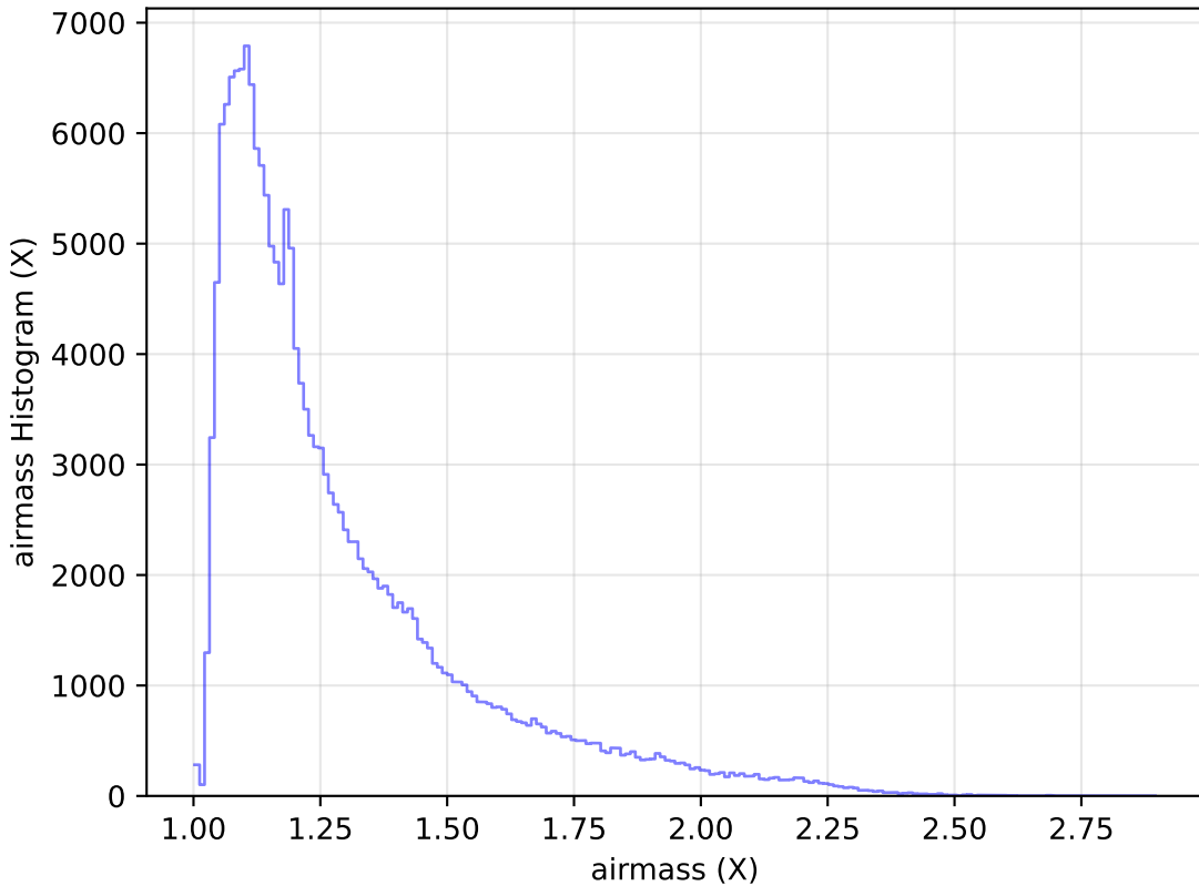
internal_u_expt27_nscale0.9v3.4_10yrs WFD g band: airmass Histogram
