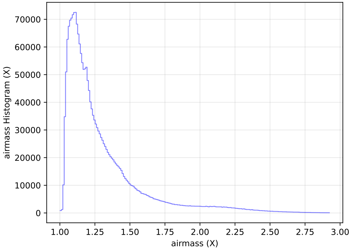
internal_u_expt27_nscale0.9v3.4_10yrs WFD all bands: airmass Histogram
