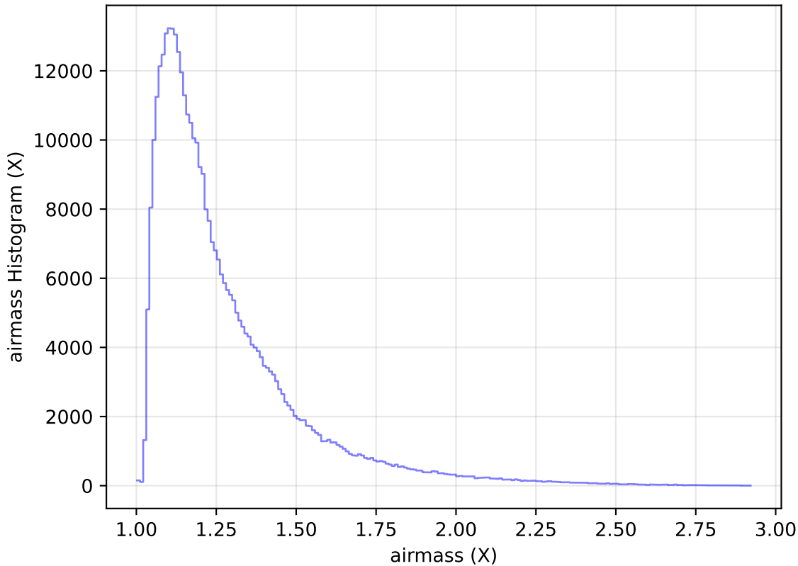
internal_u_expt27_nscale0.9v3.4_10yrs All sky y band: airmass Histogram
