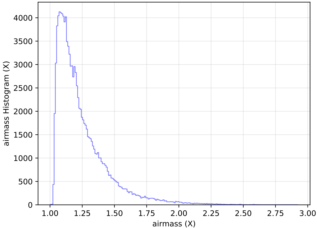
internal_u_expt27_nscale0.9v3.4_10yrs All sky u band: airmass Histogram
