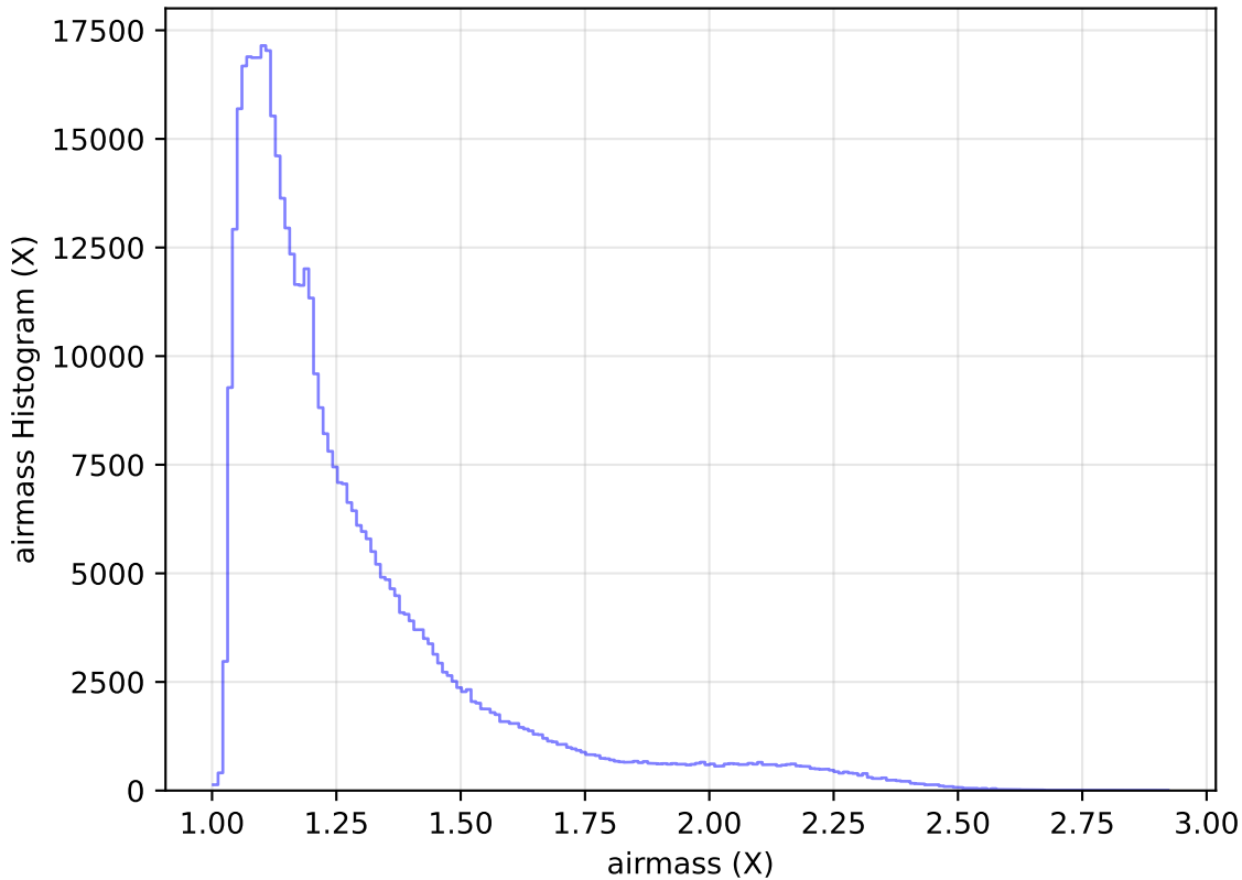
internal_u_expt27_nscale0.9v3.4_10yrs All sky r band: airmass Histogram
