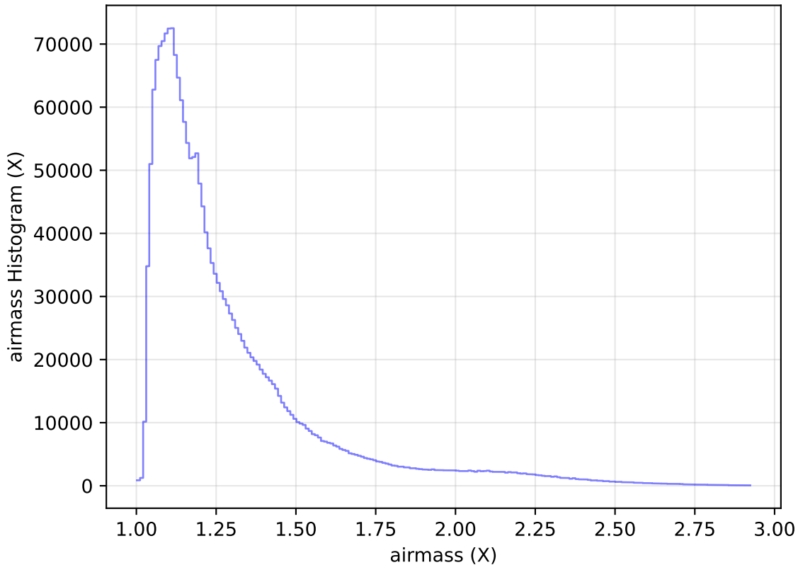
internal_u_expt27_nscale0.9v3.4_10yrs All sky all bands: airmass Histogram
