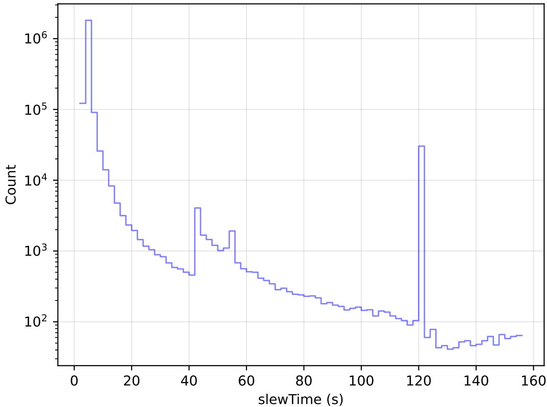
internal_u_expt27_nscale0.9v3.4_10yrs All visits: Slew Time Histogram
