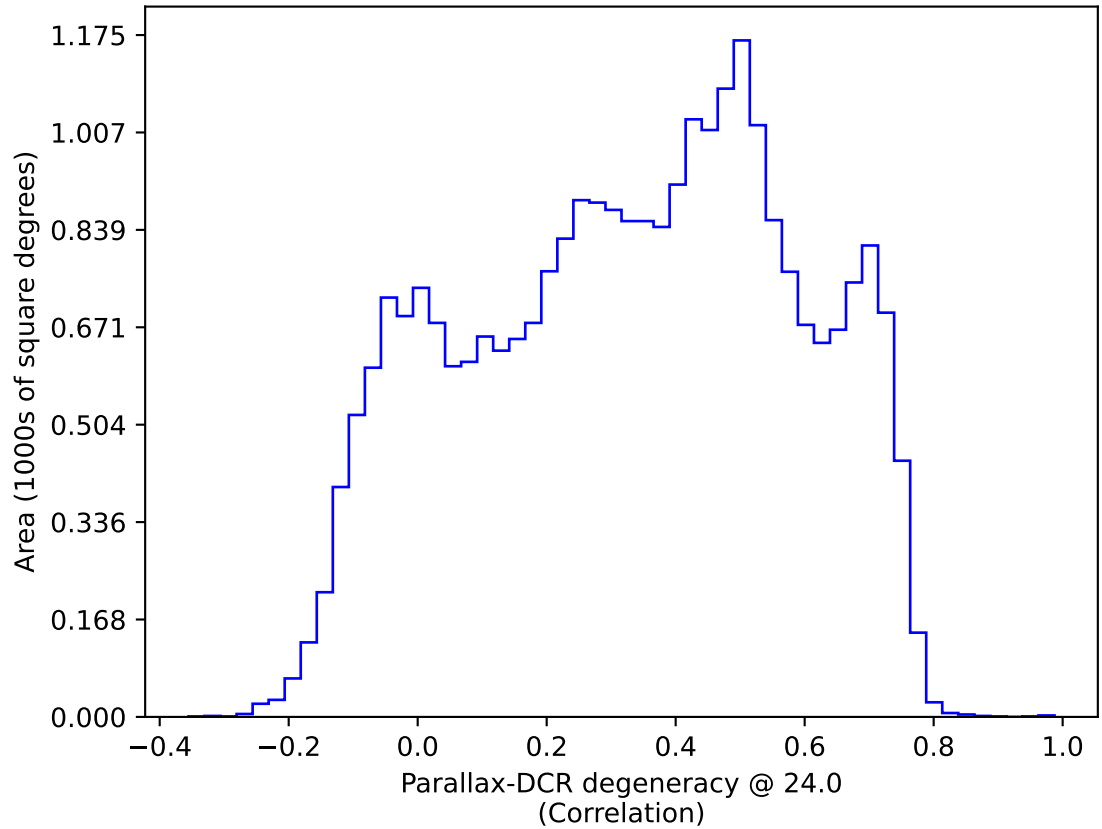
internal_u_expt27_nscale0.9v3.4_10yrs All sky: Parallax-DCR degeneracy @ 24.0
