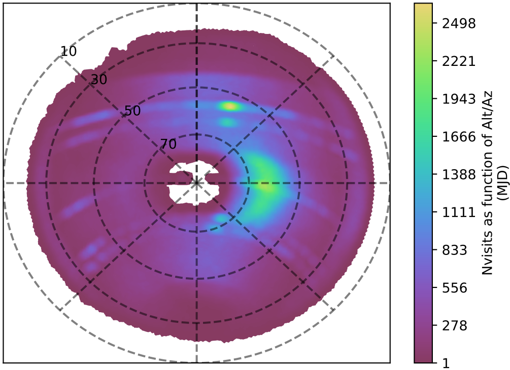
internal_u_expt27_nscale0.9v3.4_10yrs z band: Nvisits as function of Alt/Az
