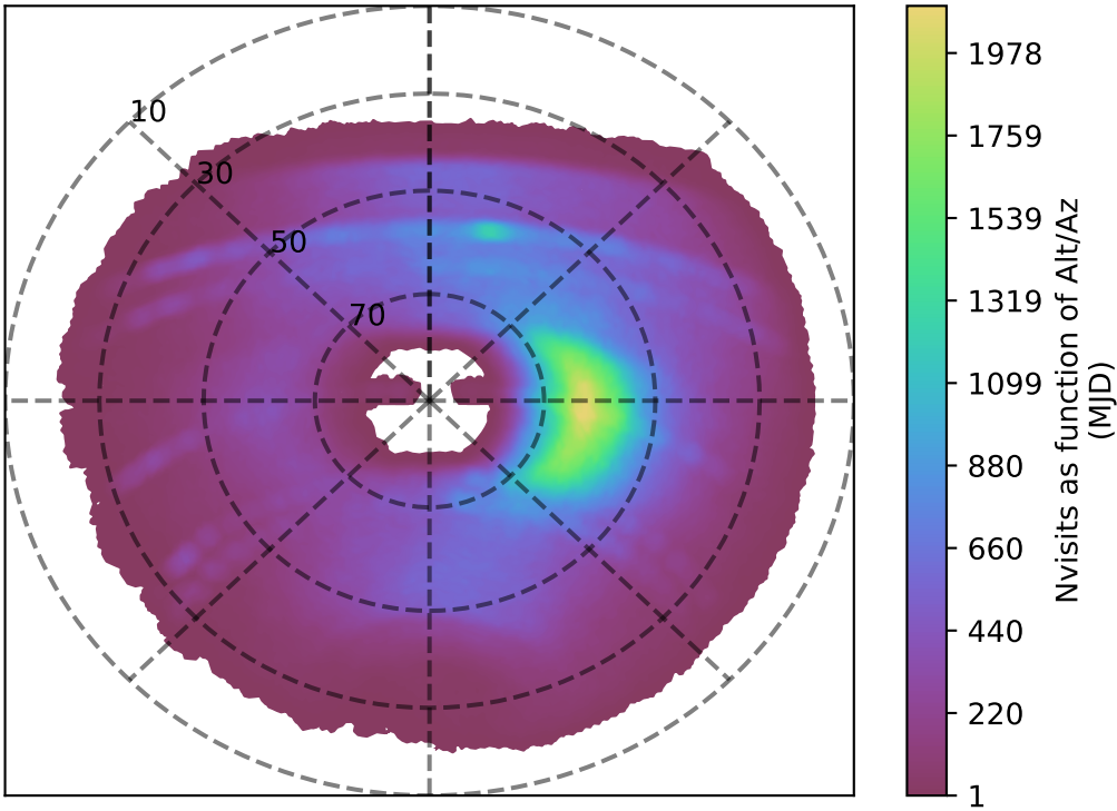
internal_u_expt27_nscale0.9v3.4_10yrs y band: Nvisits as function of Alt/Az
