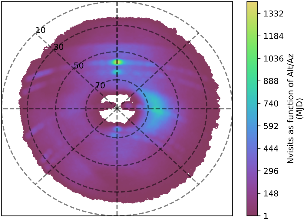
internal_u_expt27_nscale0.9v3.4_10yrs g band: Nvisits as function of Alt/Az
