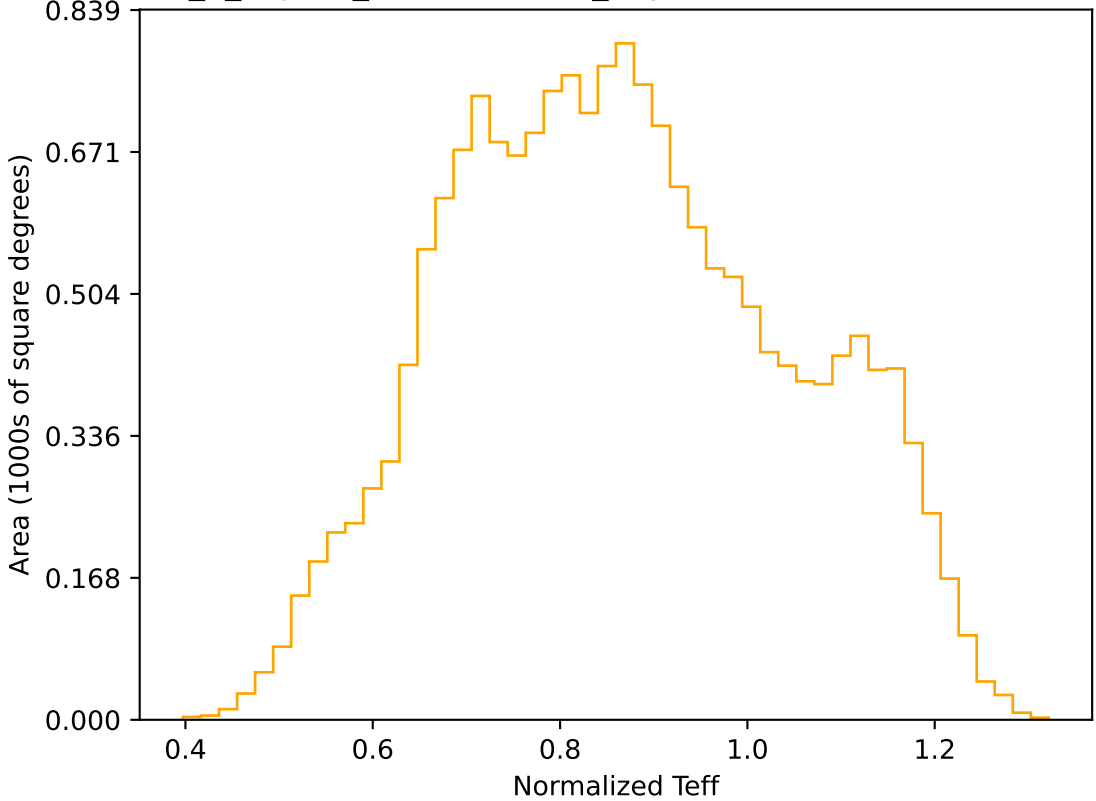
internal_u_expt27_nscale0.9v3.4_10yrs WFD r band: Normalized Teff
