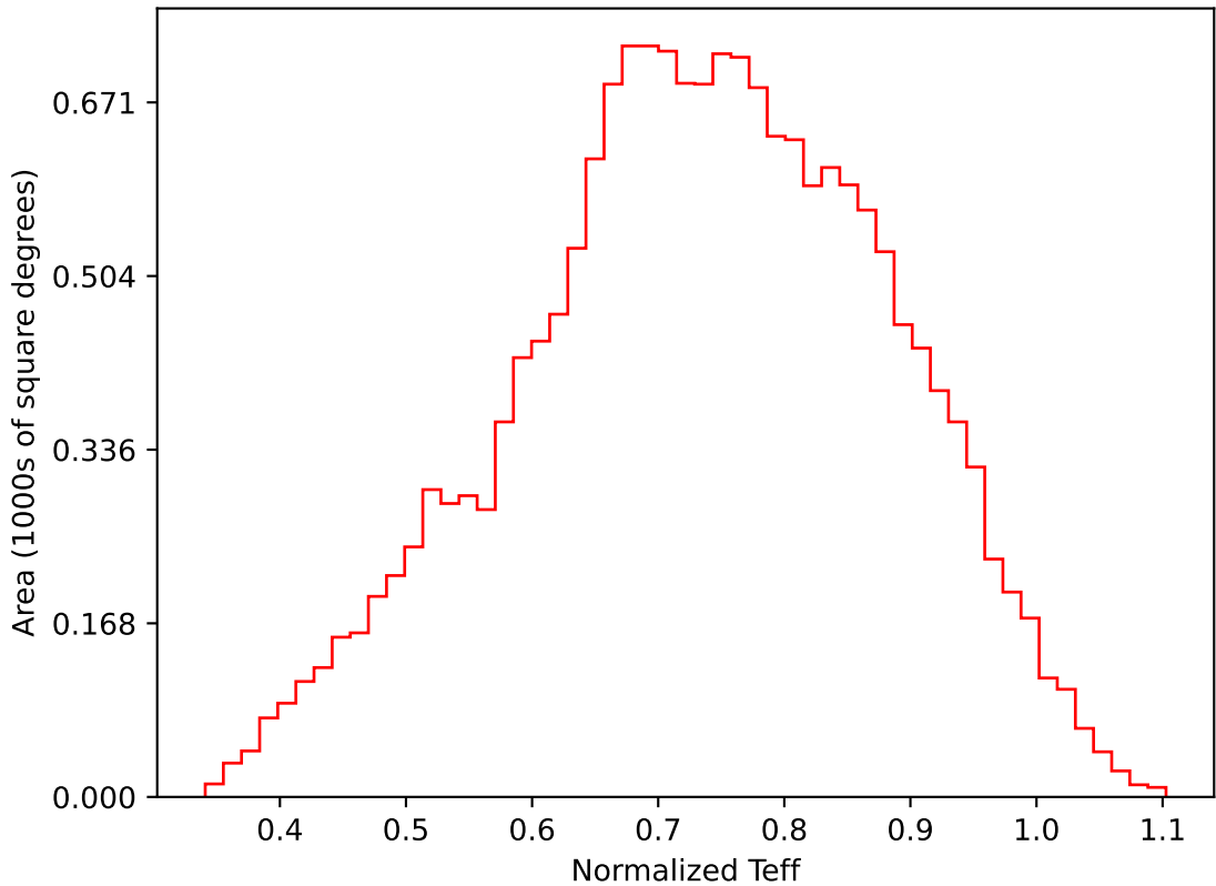
internal_u_expt27_nscale0.9v3.4_10yrs WFD i band: Normalized Teff
