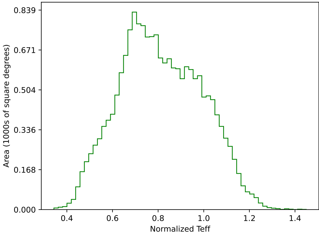
internal_u_expt27_nscale0.9v3.4_10yrs WFD g band: Normalized Teff
