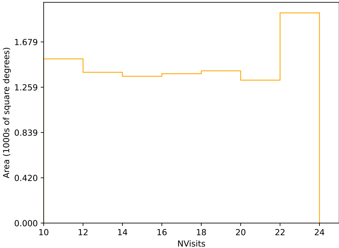
internal_u_expt27_nscale0.9v3.4_10yrs Yr 3-4 r band: NVisits
