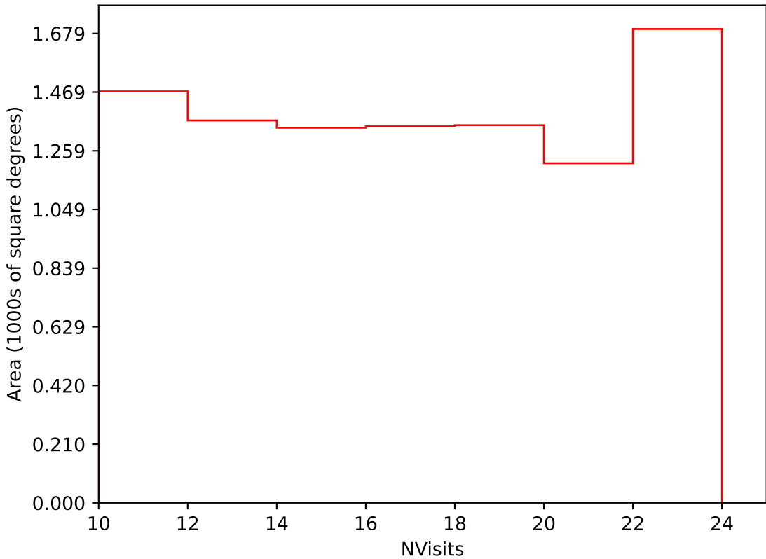
internal_u_expt27_nscale0.9v3.4_10yrs Yr 3-4 i band: NVisits
