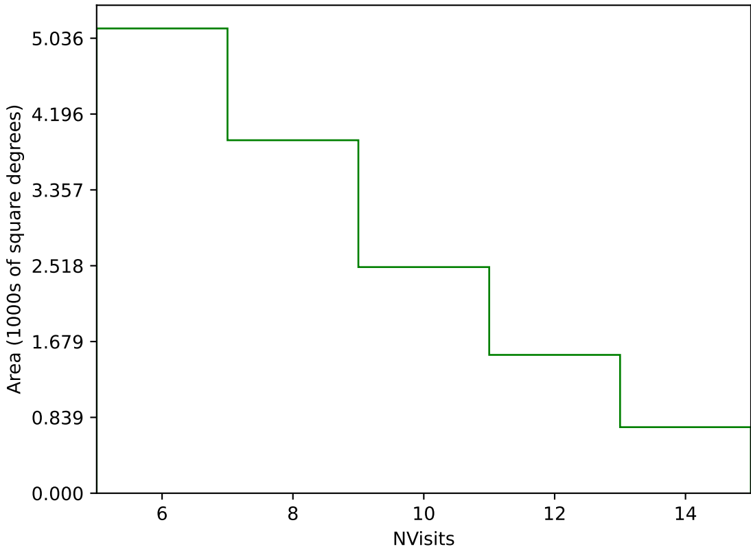
internal_u_expt27_nscale0.9v3.4_10yrs Yr 3-4 g band: NVisits
