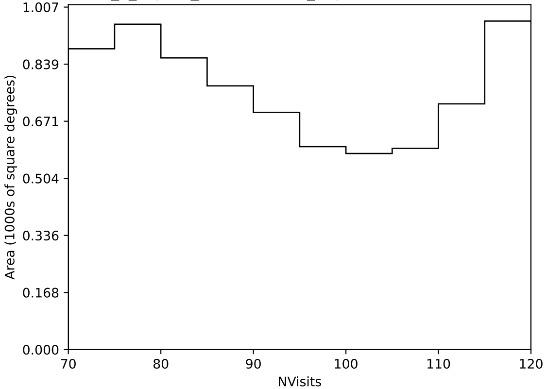
internal_u_expt27_nscale0.9v3.4_10yrs Yr 3-4 all bands: NVisits
