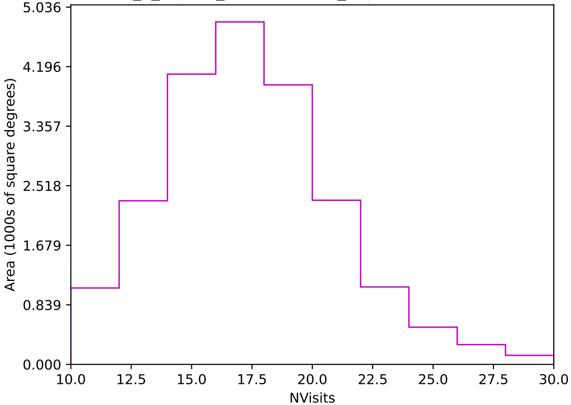
internal_u_expt27_nscale0.9v3.4_10yrs Yr 1 z band: NVisits
