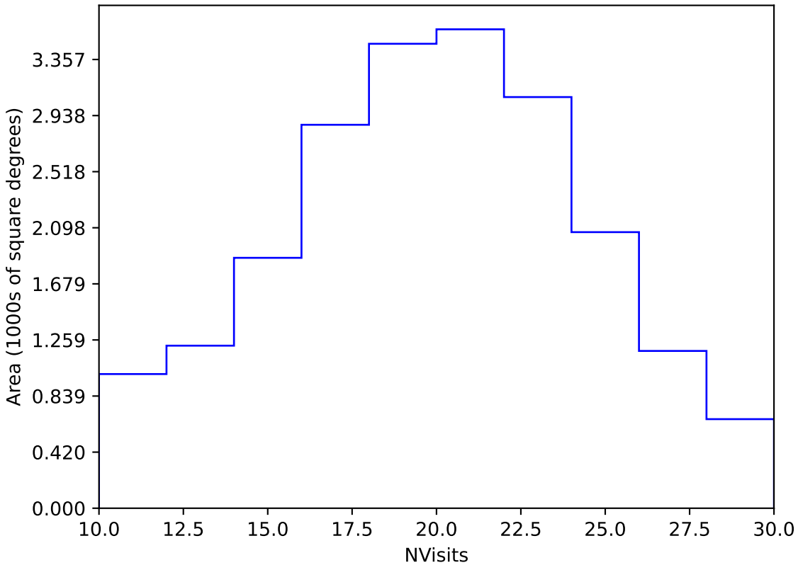
internal_u_expt27_nscale0.9v3.4_10yrs Yr 1 y band: NVisits
