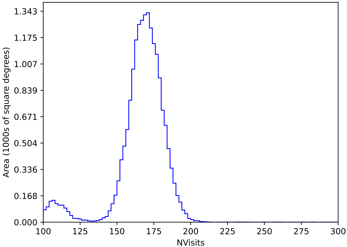
internal_u_expt27_nscale0.9v3.4_10yrs WFD y band: NVisits
