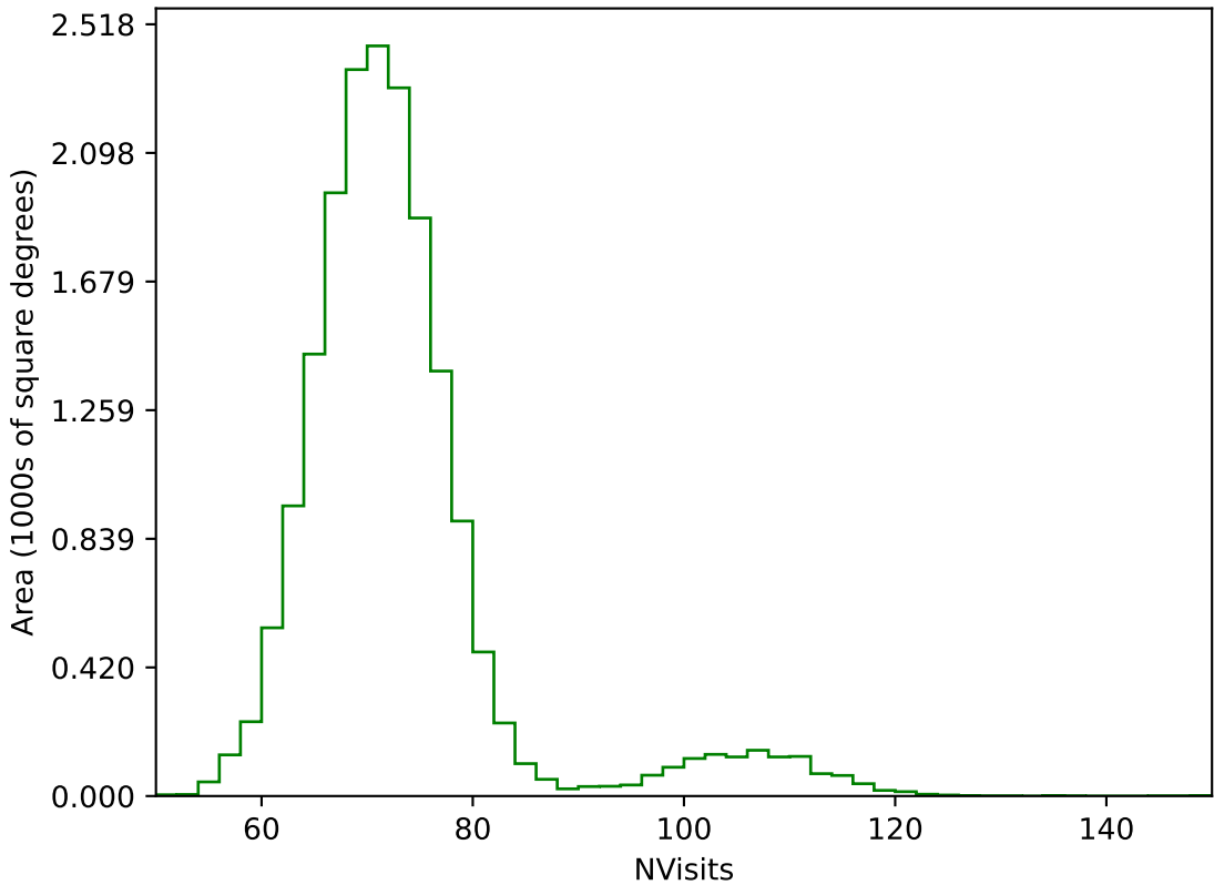
internal_u_expt27_nscale0.9v3.4_10yrs WFD g band: NVisits
