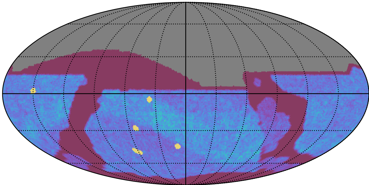
internal_u_expt27_nscale0.9v3.4_10yrs All sky z band: NVisits
